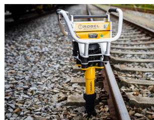
ROTAMP 62.20L E 3 Battery Powered Tie Tamper
