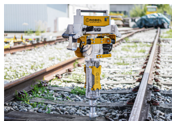
ROSPIKE 33.25 E 3 Battery Powered Spike Driver
