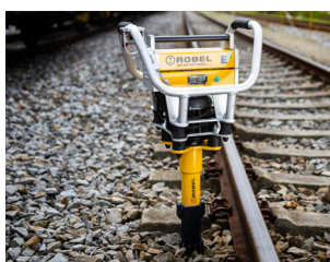
ROTAMP 62.20L E 3 Battery Powered Tie Tamper
