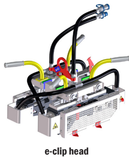
e-clip head
