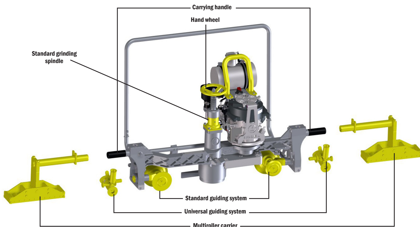
Illustration ROGRIND 13.45SKS: Left-hand guide handle
